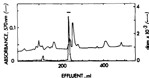
Fig. 2. Elution profile of the tryptic peptides of CNBr fragment E from chromatography on Dowex 50-X8. Thiol group III was labelled with [^{14}\text{C}] cyanide.
